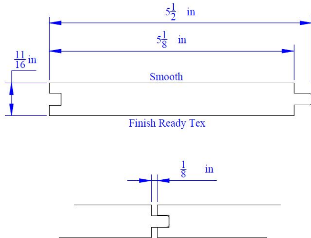
Vertical Grain T&G Patterns - T&G Rev. Finline Smooth/Finish Ready (24G)
