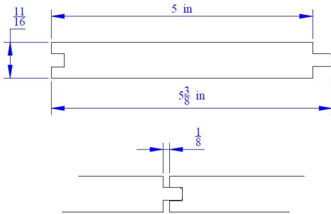
Vertical Grain T&G Patterns - Thermally Modified T&G Rev. Finline RS/Finish Ready
