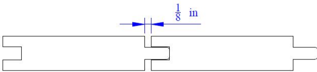
T&G and Shiplap Patterns - Rev. Finesline Resawn/Smooth
