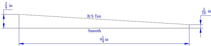
Clear Bevel - KD VG wRC Resawn/Smooth Back
