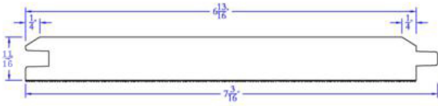
T&G and Shiplap Patterns - WP4 Face / Flush Resawn Back
