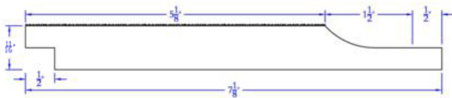
T&G and Shiplap Patterns - Shiplap 771 Cove Resawn Face
